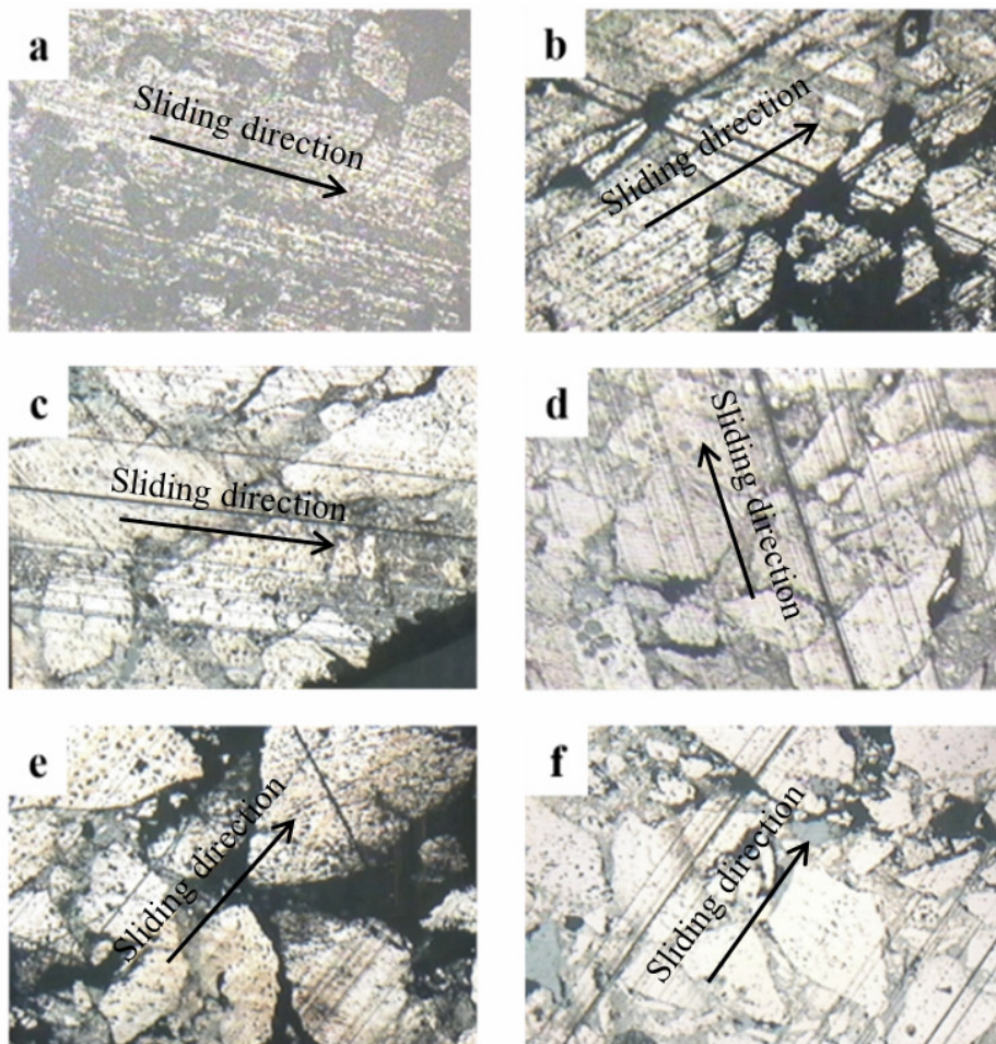
Figure 6 Digital microscope images of worn surfaces of PKAC-E composite testing at (a) 5N, (b) 20N, (c) 40N, (d) 60N, (e) 80N and (f) 100N
