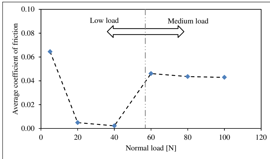
Figure 3 Relationship between applied loads and average friction coefficient of PKAC-E composite
