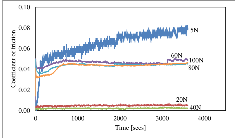
Figure 4 Comparison of friction coefficient as a function of time at different load
