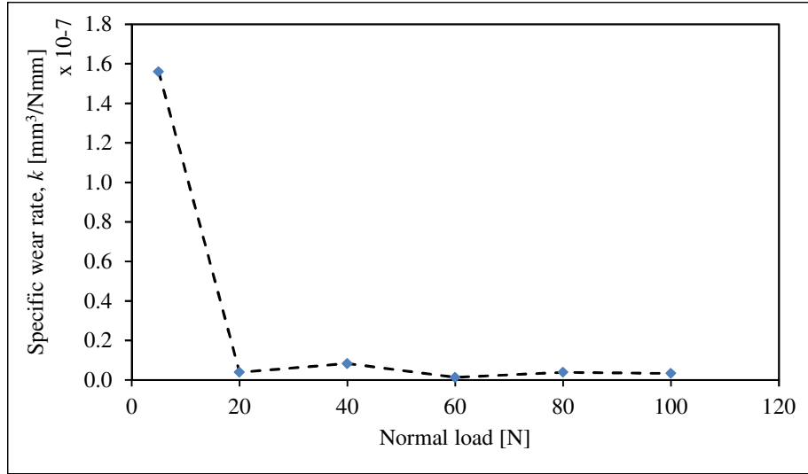
Figure 5 Relationship between applied loads and wear rate of PKAC-E composite
