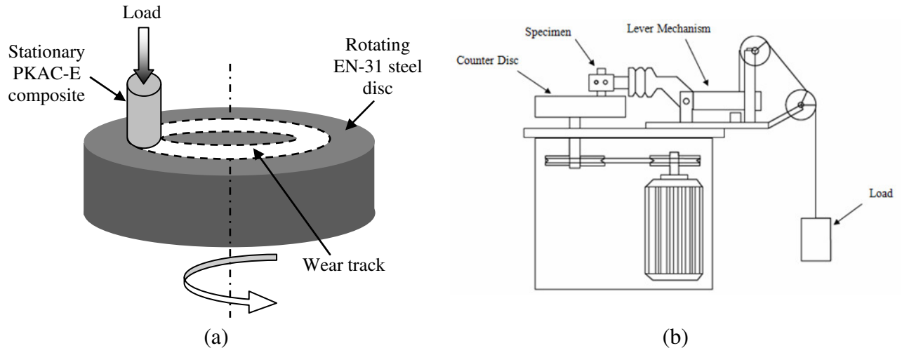
Figure 2 (a) Illustration and (b) schematic diagram of the sliding test using a pin-on-disc tribometer
